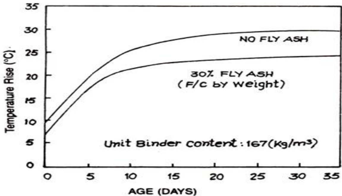
Fig. 6.12. Change in rate of the heat evolution of concrete with and without fly ash
